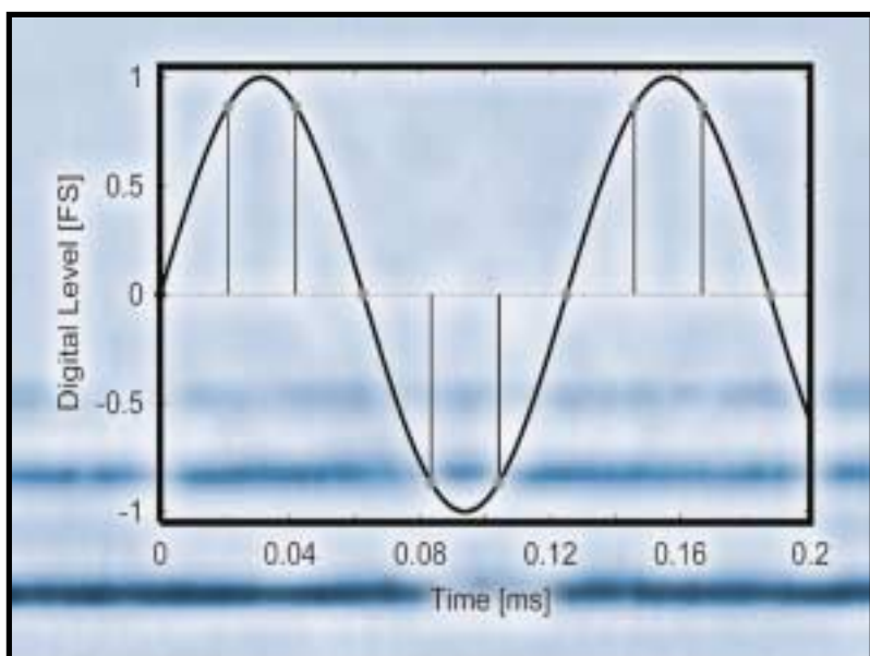
Figure 3. Digital Vs analogue level. 8kHz sine at 48kHz sampling.
