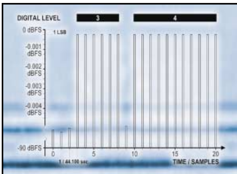
Figure 2. The samples of Figure 1 with 1dB of boost, minus 1 LSB.
