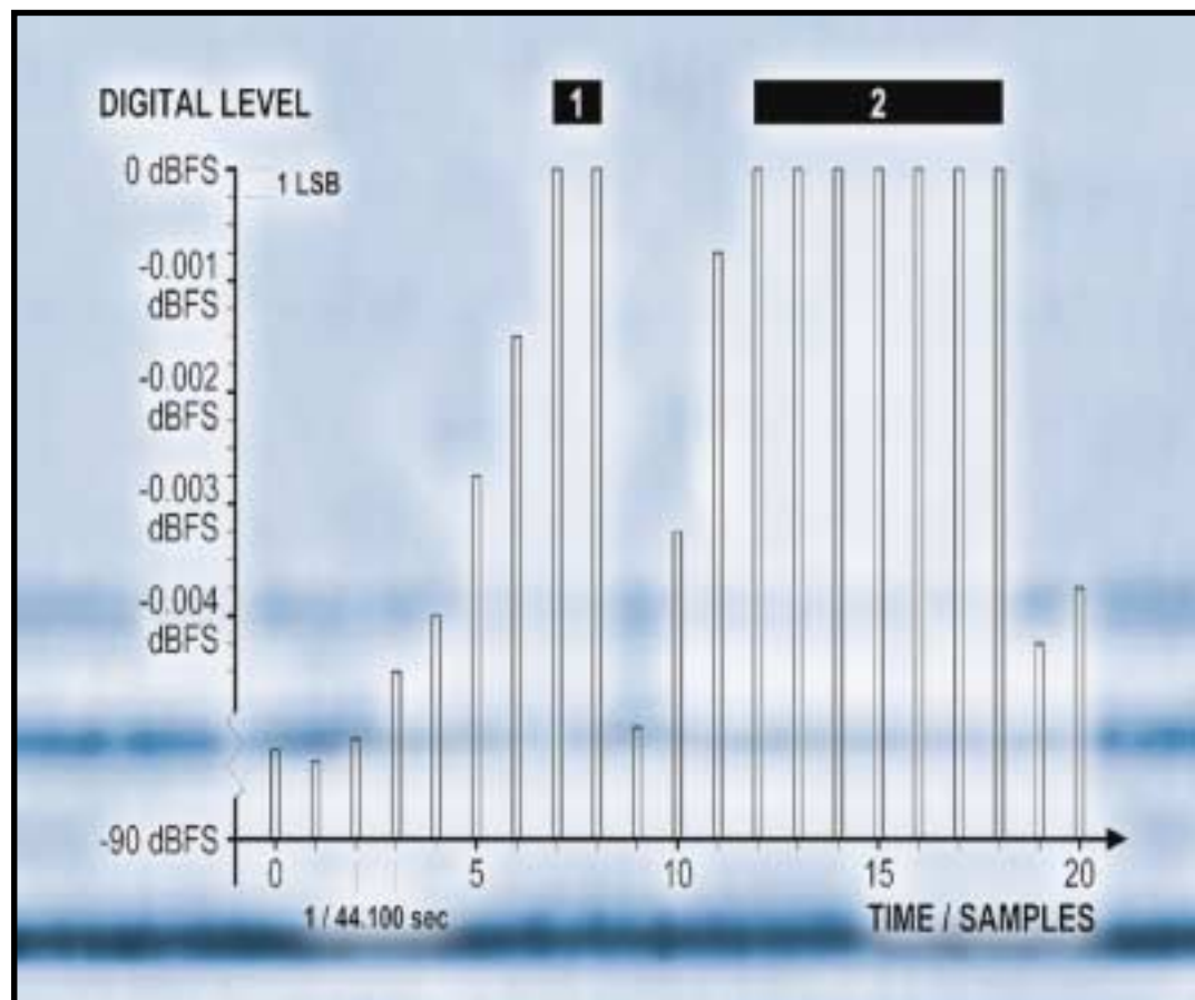
Figure 1. Example of consecutive samples on a CD.
